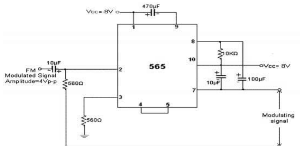
Fig 11.3: FM Demodulation circuit diagram using IC 565
