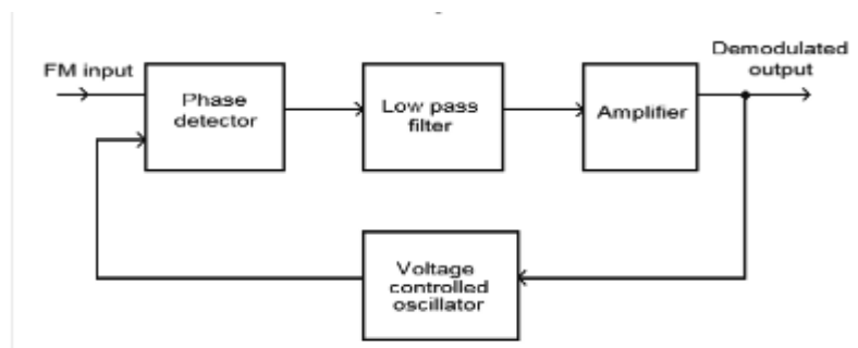
Fig 11.1 PLL block diagram
