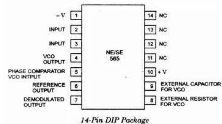
Fig 11.2 IC 565 Pin diagram
