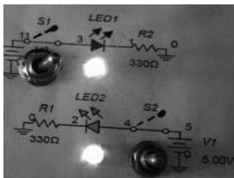
Fig 2.5: Experimental set up of Full duplex used in laboratory when S1 and S2 is closed
