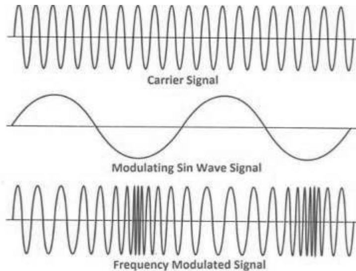
Fig 6.2: FM waveforms
