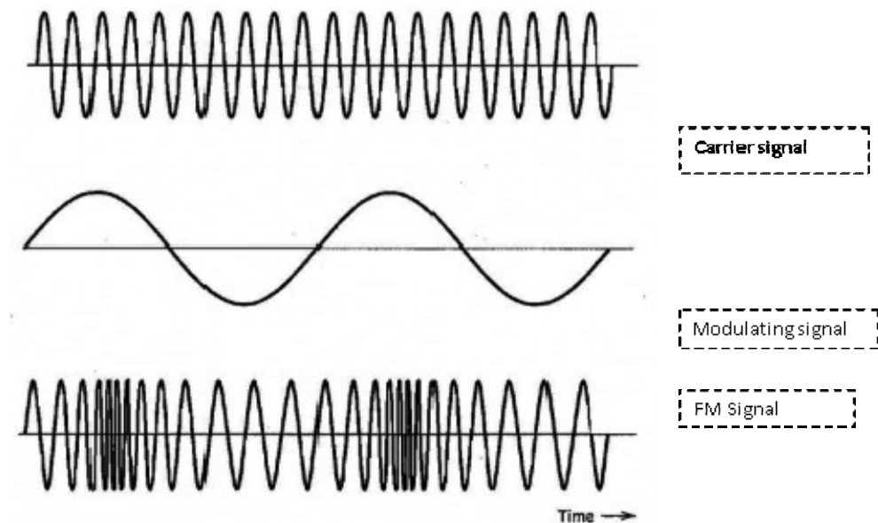
Fig 8.1: FM waveforms
