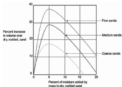
Bulking of Aggregate
