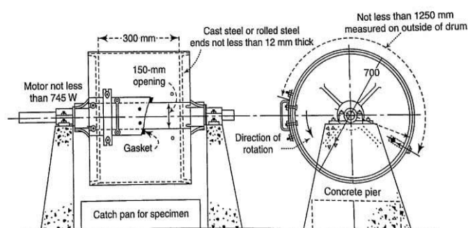
Figure: Los Angeles Abrasion Testing Machine
