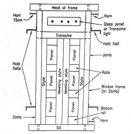
Figure 12: Component parts of door and window
