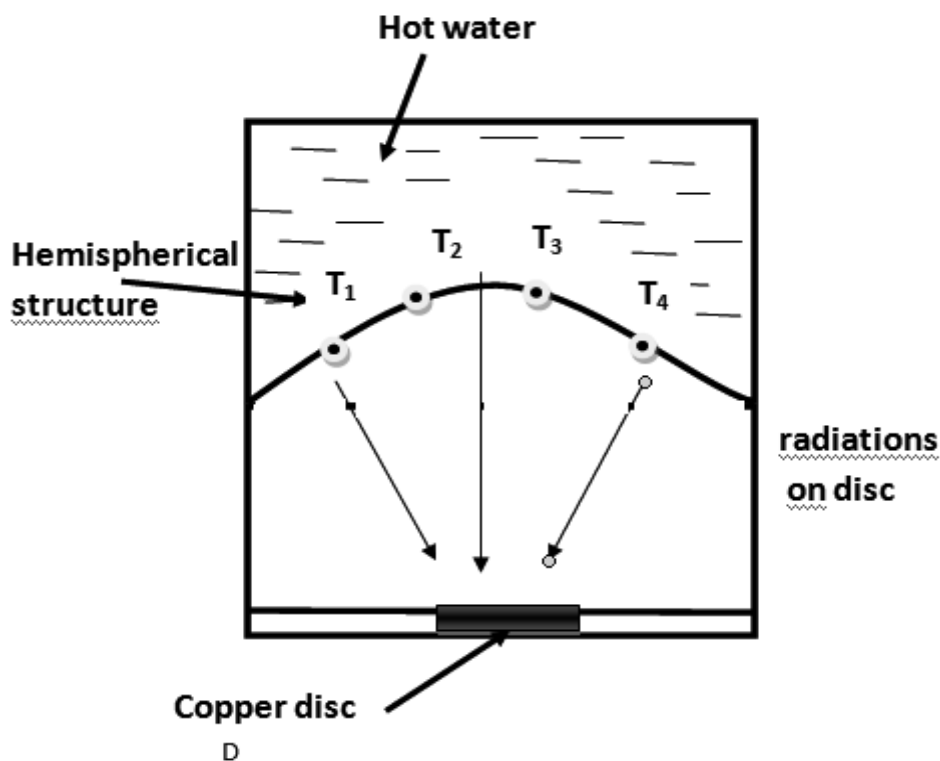
D Experimental setup for Stefan Boltzmann law
