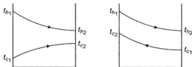
Parallel flow
